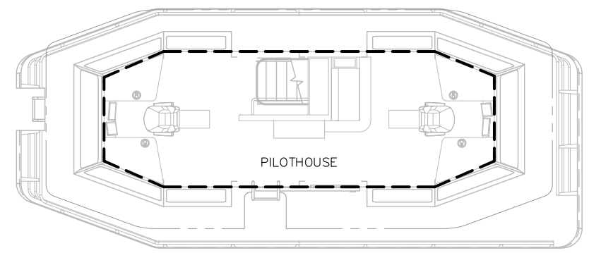
PLAN 4-7A PILOTHOUSE DECK BULKHEADS 1/8"=1'-0"
