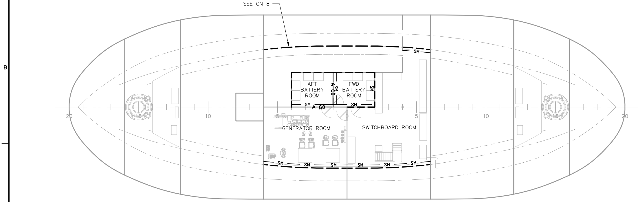
PLAN 2-5C HOLD DECK BULKHEADS 1/16"=1'-0"
